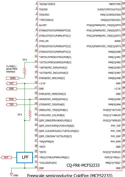
Freescale semiconductor ColdFire (MCF52233) MIDI FM tone generator TGMCF for CQ-FRK-MCF52233 board (CQ Publishing) Minimal configuration 2008/8/24
