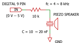
(c) Piezo speaker with resistor
