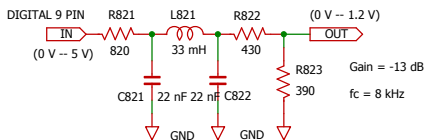
(b) 3rd order passive LC filter ( Z_o = 820 \text{ Ohm} , f_c = 8 \text{ kHz} )
